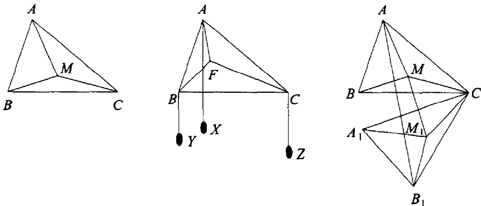
FIGURE 4.16. Fermat's point.
