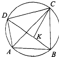
FIGURE 4.3 . Ptolemy's theorem.
